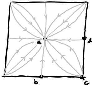
FIGURE 1. An example of gradient flow on the torus.
